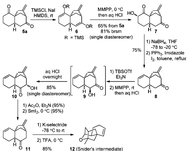
Scheme 2. Formal Formal Synthesis of (±)-Platensimycin 1
