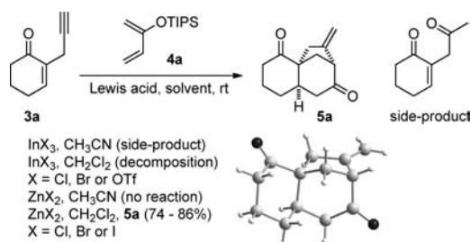
Scheme 1. Screening of Bifunctional Lewis Acids
