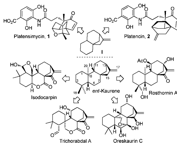
Figure 1. Examples of ent -kaurene related natural products.
